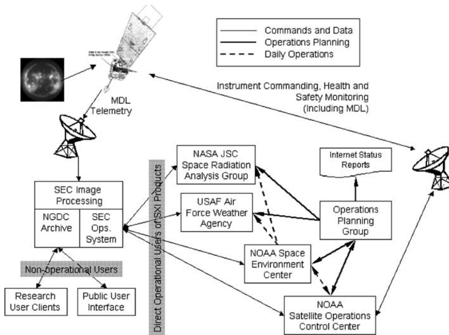
Figure 5. SXI operation concept.
