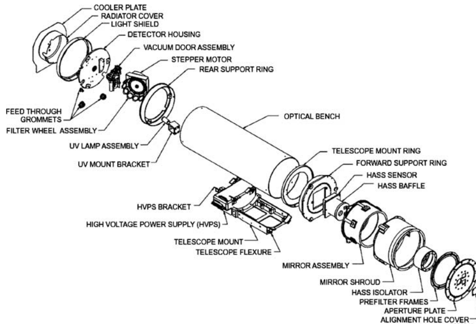
Figure 2. Instrument exploded view (GOES I-M Data Book (1996)).
