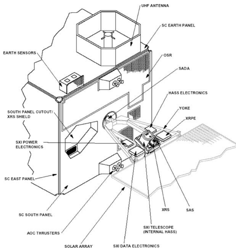
Figure 1. Instrument mounting configuration (GOES I-M Data Book (1996)).
