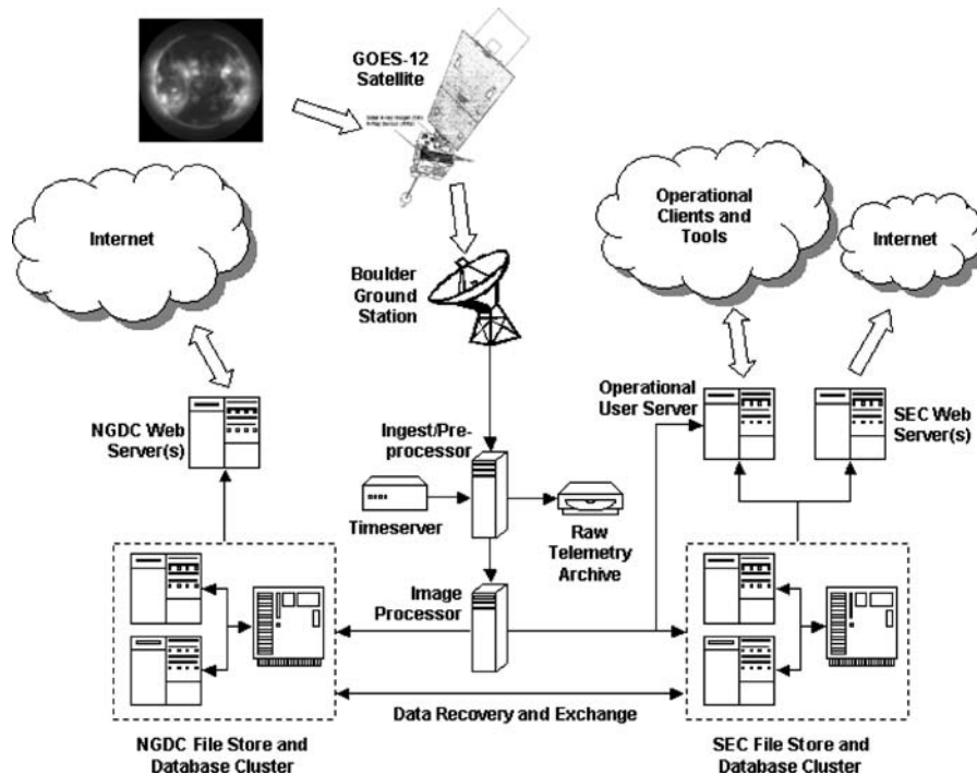
Figure 6. Ground data system.
