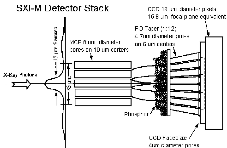
Figure 3. Detector stack schematic (Bornmann et al. , 1997).
